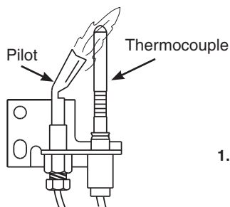
Pilot Assembly Fig. 11-1
